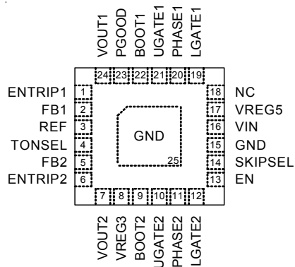
RT8205A WQFN-24L 4x4
